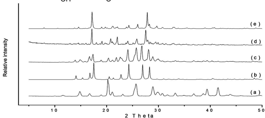
Fig. 15 Demonstration of the enhanced kinetics of cococrystal formation upon addition of a few drops of methanol to the grinding jar. PXRD patterns for (a) tetracarboxylic acid, (b) bipirydil, (c) outcome of neat grinding for 60 minutes (as the sum of the reactants), (d) the product obtained when a few drops of methanol are added and (e) the simulated pattern for the cococrystal.
