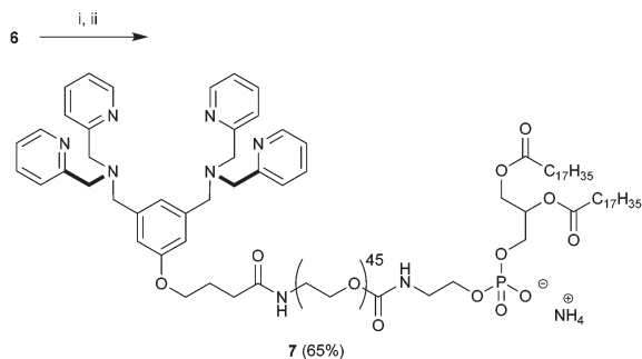
Scheme 2 Preparation of BDPA-PEG 2000 -DSPE ( 7 ). Conditions: (i) PfpOH, EDC, DMAP, \text{CHCl}_3 , 0^\circ\text{C} to rt, 16 h followed by (ii) H 2 N-PEG 2000 -DSPE, DIPEA, \text{CHCl}_3 , rt, 24 h.
