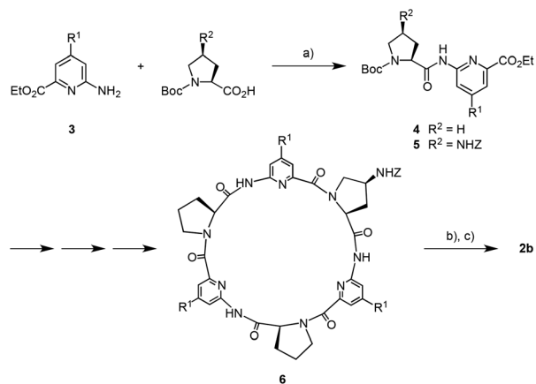
Scheme 1 Synthesis of bis(cyclopeptide) 2b (R 1 = (OCH 2 CH 2 ) 3 OCH 3 ). (a) Chlorotripropylidiphosphonium hexafluorophosphate (PyCl 6 ), N,N -diisopropylethylamine, CH 2 Cl 2 , 25 °C, 10 d, 4 82%, 5 96%; (b) H 2 , 1.2 equiv. HCl, 10% Pd/C, CH 2 Cl 2 –CH 3 OH, 1 : 1 (v/v), 25 °C, 18 h; (c) 2,2'-(1,3-phenylene)diacetic acid, 2-(1 H -benzotriazole-1-yl)-1,1,3,3-tetramethyluronium (TBTU), N,N -diisopropylethylamine, dimethylformamide, 25 °C, 2 h, 47% over 2 steps. Z = benzyloxy carbonyl, Boc = tert -butoxy carbonyl.
