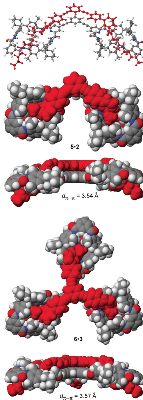
Fig. 1 MM2 force field-optimized structures of the divalent and trivalent pseudorotaxanes 5·2 and 6·3 . Space-filling representations provide top and side views.
