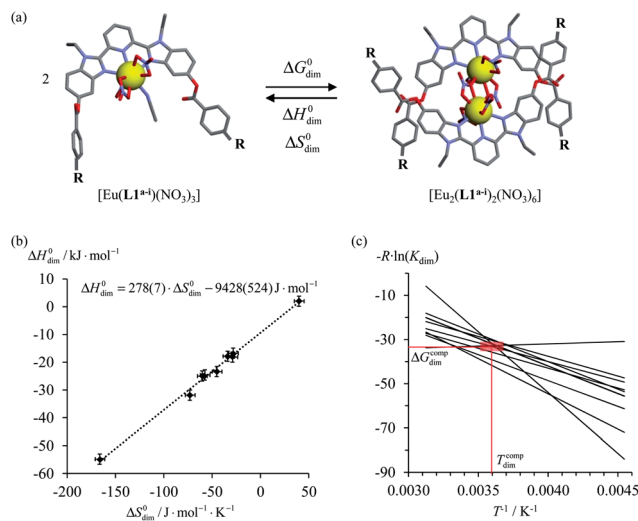
Fig. 1 (a) Schematic dimerization of complexes [\text{Eu}(\text{L1}^{2-})(\text{NO}_3)_3] occurring in dichloromethane, (b) associated "linear" \Delta H_{dim}^0 vs. \Delta S_{dim}^0 plots and (c) individual van't Hoff \Delta G_{dim}/T vs. T^{-1} plots for nine different R substituents. 15
