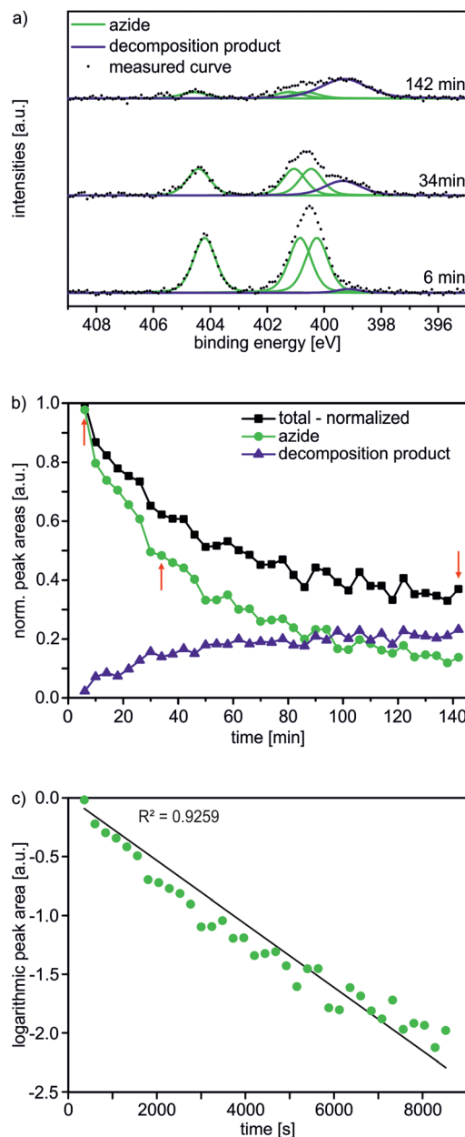
Fig. 1 In situ damage of the AUD SAM caused by monochromatic Al K\alpha radiation (X-ray excitation energy 1486 eV) with (a) peak fits of the N 1s XP spectra, (b) quantitative analysis of the individual peak fits. Red arrows indicate the data points corresponding to the spectra in (a). (c) Logarithmic plot of normalised azide peak areas over time. All peak areas are normalized to the total peak area of the first spectrum after 6 min irradiation time.
