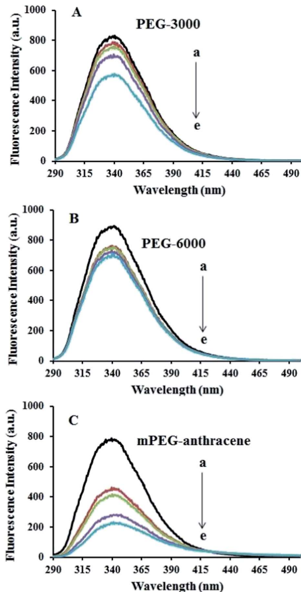
Fig. 1 Fluorescence emission spectra of \beta -LG in 10 mM Tris-HCl under varying concentrations of (A) PEG-3000, (B) PEG-6000 and (C) mPEG-anthracene. \lambda_{\text{ex}} = 295 nm. T = 298.15 K, pH 7.4, [\beta\text{-LG}] = 30 \mu\text{M} . The concentrations of polymers from (a) to (e) are 0, 15, 25, 35 and 45 \mu\text{M} , respectively.
