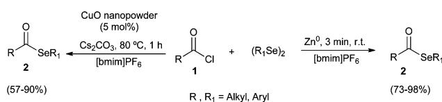
Scheme 7 Preparation of selenol esters in ionic liquid (IL).
