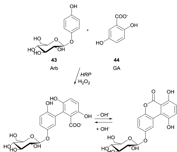
Scheme 13 Coupling of 4'-hydroxyphenyl-β-D-glucoside (arbutin, Arb) (43) with 2,5-dihydroxybenzoic acid sodium salt (gentsiate, GA) (44).
