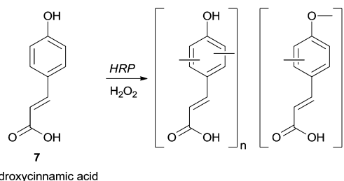
Scheme 2 Chemoselective polymerization of p -hydroxycinnamic acid ( 7 ).
