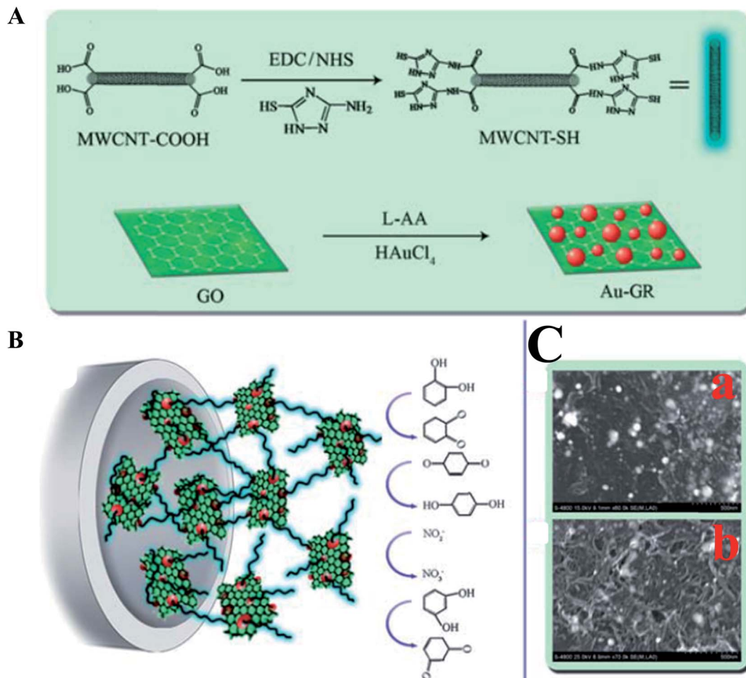
Fig. 9 (A) Preparation process for MWCNT-SH and Au-GR. (B) Schematic depiction of the MWCNT-SH@Au-GR electrode. (C) SEM images of Au-GR nano hybrid (a) and MWCNT-SH@Au-GR hybrid material (b). Reproduced with permission from ref. 161 © 2013 Royal Society of Chemistry.
