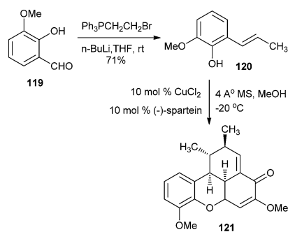
Scheme 27 Synthesis of benzoxanthene 121 .
