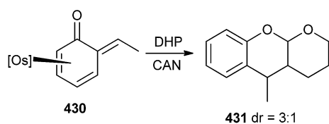
Scheme 93 Reaction of Os-complexed o -QM with 3,4-dihydropyran.
