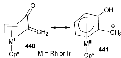
Scheme 96 Resonating forms of metal o -QM complex.
