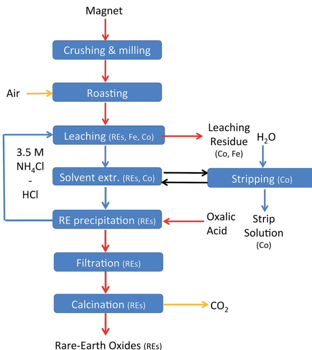
Fig. 14 Flow chart of the recycling scheme. Yellow arrows: gas steams, blue arrows: aqueous streams, black arrows: ionic liquid stream, and red arrows: solid streams.
