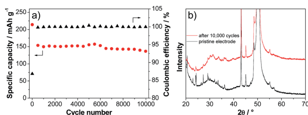
Fig. 6 (a) Long-term cycling performance of LVP anodes cycled between 3.0 and 0.0 V vs. Li/Li + at a current corresponding to 50 C. (b) XRD pattern of a pristine electrode and the electrode subjected to 10 000 cycles at 50 C.
