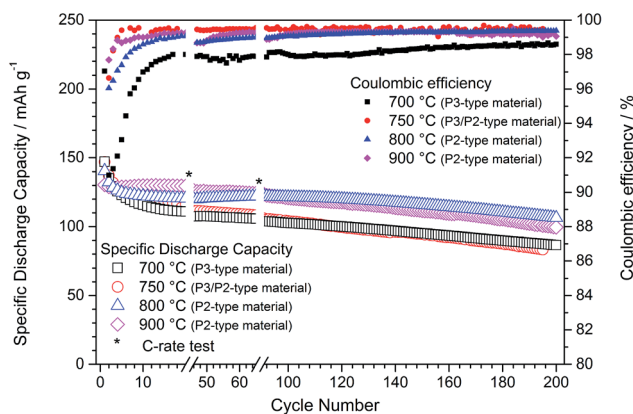
Fig. 4 Specific discharge capacity vs. cycle number of \text{Na}_x\text{Ni}_{0.22}\text{Co}_{0.11}\text{Mn}_{0.66}\text{O}_2 annealed at 700, 750, 800 and 900 °C. Cut-off limits: 4.3–2.1 V (vs. Na/Na + ). Reference and counter electrodes: Na. Electrolyte: 1 M NaPF 6 in PC. Temperature: 20 ± 2 °C. Cycles 1–20, 46–50, 91–200 were performed at 0.1 C (12 mA g -1 ). During cycles 21–45 and 65–90 a C-rate test was performed from 0.1 C (12 mA g -1 ) to 5 C (615 mA g -1 ).
