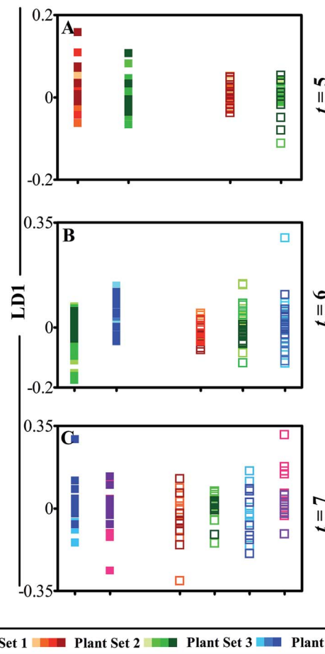
Fig. 3 Cross-validated PCA-LDA 1D scores plot of ATR-FTIR spectra obtained over a three week period ( t = weeks 5, 6 and 7 of development) to distinguish spectral effects of the technique. Each square corresponds to an individual spectrum, and colour variation indicates advancing time points through the respective time frame. Full squares (■) represent a comparison between leaflets specifically analysed the previous week with equivalent leaflets from a newly introduced plant set, and empty squares (□) compare a newly expanded leaflet to observe any systemic effects as well as local effects of the technique. (A) Compares previously analysed leaflet A and systemic leaflet B in plant sets 1 and 2; (B) leaflets B and C and (C) leaflets C and D.
