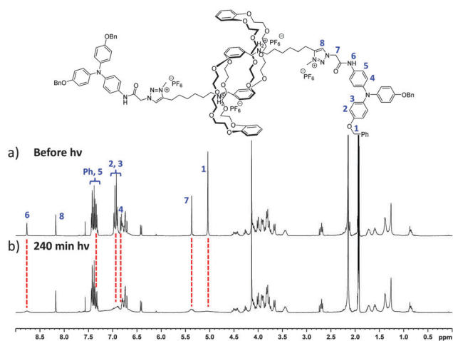
Fig. 1 Typical 1 H NMR spectra of 7 obtained immediately after purification (a) and after 4 hours of exposure to a 20 W power halogen lamp (b), [7] ≈ 5 mM in CD 3 CN with 2.5% CDCl 3 . The red lines indicate the disappearance of the characteristic triarylamine signals upon light irradiation.
