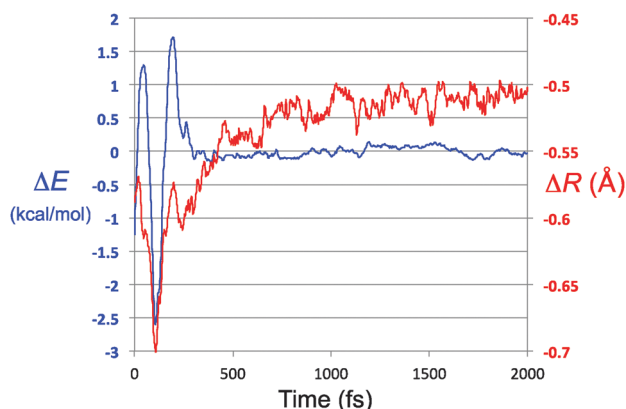
Fig. 7 Overlay of the energy residual trace for TFIPA, from Fig. 6 ( \Delta E axis and blue trace on this graph) and the closest approach of solute and solvent atom pairs, with respect to the sum of their van der Waals radii ( \Delta R axis and red trace).
