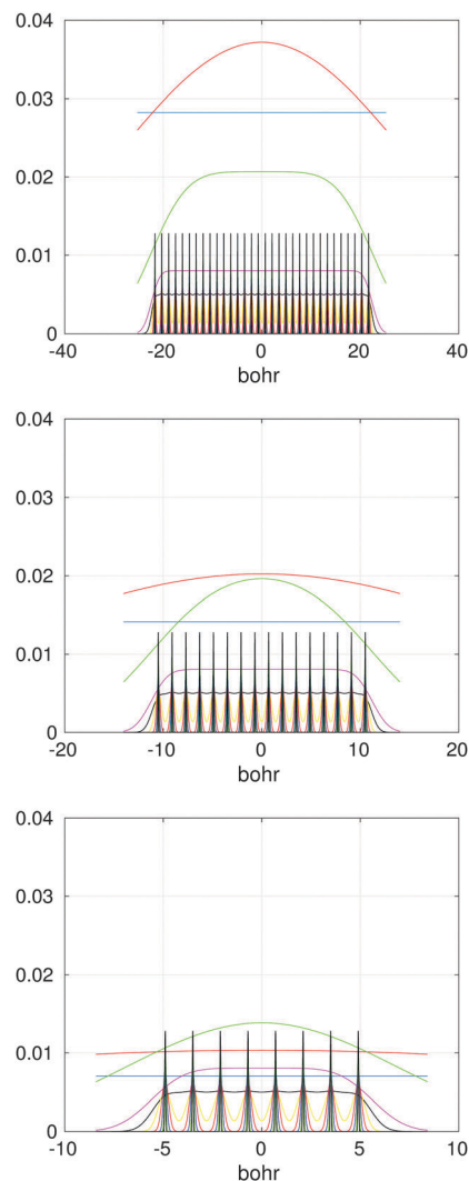
Fig. 15 Assembled x-, y- and z-axis canonical vectors for a cluster of 32 \times 16 \times 8 hydrogen atoms.
