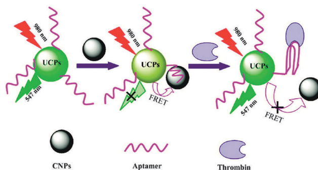
Fig. 17 Scheme of the design and function of a thrombin sensor based on UCNP. An aptamer on the UCNP surface binds to a carbon nanoparticle (CNP) via weak \pi - \pi interactions. The CNP quenches the upconversion emission by FRET. Thrombin changes the structure of the aptamer, releases the CNP from the UCNP surface and thus restores the upconversion emission. Reprinted with permission from ref. 38. Copyright © 2011, American Chemical Society.
