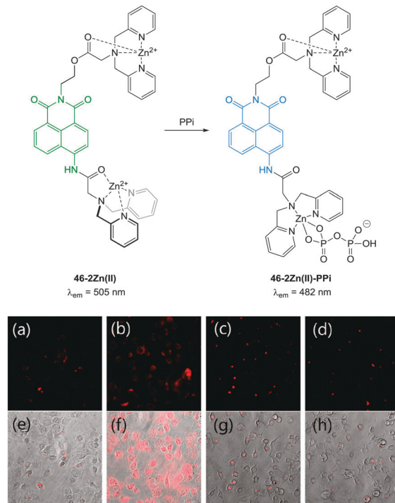
Fig. 39 (a) Fluorescence image of C2C12 cells treated with 46-2Zn(II) (1.0 \mu M). (b) Fluorescence images of C2C12 cells treated with 46 (1.0 \mu M) and Zn(II) (5.0 \mu M). (c) Fluorescence images of C2C12 cells treated with 46 (1.0 \mu M), Zn(II) (5.0 \mu M) and PPI (0.5 mM). (d) Fluorescence images of C2C12 cells treated with 46 (1.0 \mu M), Zn(II) (5.0 \mu M) and PPI (1.0 mM). (e–h) Bright field images of (a–c) respectively. Image reproduced with permission. 190
