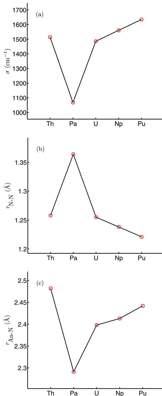
Fig. 3 N–N stretching wavenumber (a), r(\text{N}-\text{N}) (b) and r(\text{An}-\text{N}) (c) for [\text{An}(\text{OPh})_3]_2(\mu-\eta^2:\eta^2-\text{N}_2) (An = Th–Pu).
