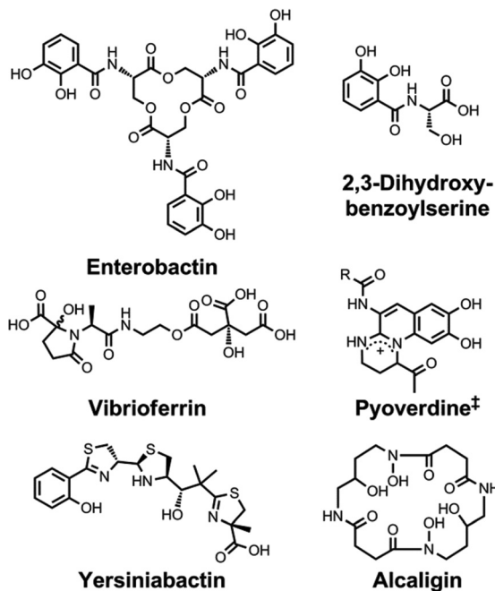
Chart 6 Chemical structures of the siderophores discussed in Siderophores as Signalling Molecules . The stereochemistry of yersiniabactin was taken from ref. 31. ‡Many pyoverdines exist and are distinguished by the nature of the peptide chain attached at the R position. The chemical structure of vibrioferrin was obtained from ref. 144.
