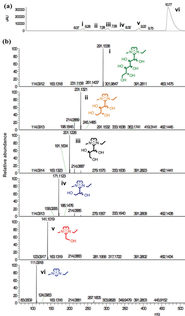
Fig. 4 LCMS investigation of adduct species formed from [C 2 C 1 im] + [OAc] - , 1a + 10 wt% D-(+)-glucose, 12 , heated to 120 °C for one hour (t 1 ): (a) survey of peaks i–vi; (b) ESI mass spectra of peaks i–vi.
