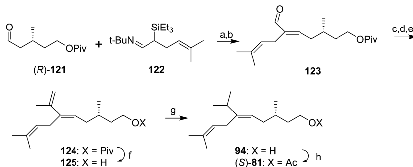
Scheme 17 Baudouy and Sancho's synthesis of yellow scale pheromone. Reagents and conditions: (a) s -BuLi, THF, -78-0^\circ\text{C} , then \text{CF}_3\text{COOH} and water, 66%; (b) pyridinium hydrochloride, \text{CH}_2\text{Cl}_2 , 100%; (c) MeMgI, ether, -70 to -35^\circ\text{C} ; (d) (\text{COCl})_2 , DMSO, \text{Et}_3\text{N} , \text{CH}_2\text{Cl}_2 ; (e) \text{MePh}_3\text{PBr} , BuLi, THF, 20^\circ\text{C} -reflux; 90% from the aldehyde; (f) DIBAL, solvent not stated, quantitative; (g) (\text{Ph}_3\text{P})_3\text{RhCl} , \text{H}_2 , benzene, quantitative; (h) \text{Ac}_2\text{O} , \text{Et}_3\text{N} , solvent not stated, 94%.
