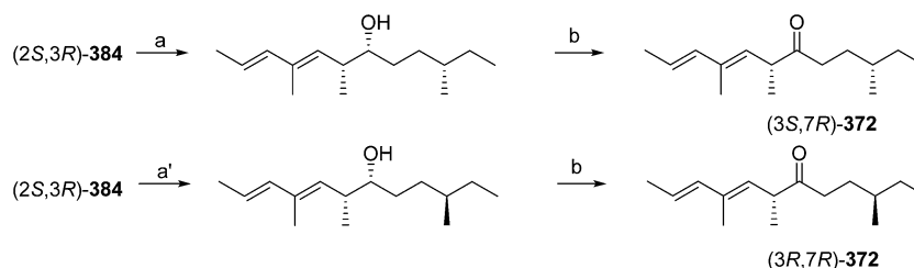
Scheme 59 Cywin's enantioselective synthesis of (3S,7R)-372 and (3R,7R)-372. Reagents and conditions: (a) (S)-2-methylbutylMgBr, CuI, THF, 60%; (a') (R)-2-methylbutylMgBr, CuI, THF, 58%; (b) ( n -Pr) 4 NRuO 4 , NMO, 4A sieves, CH 2 Cl 2 .
