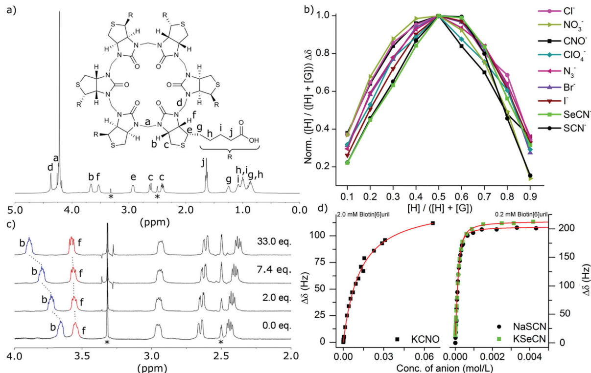
Fig. 2 (a) 1 H NMR spectrum of Biotin[6]juril. (b) Job plots for a series of anions with Biotin[6]juril. Plots are constructed using 1 H NMR data performed in 100 mM phosphate buffer pH 7.5 in D 2 O. The normalized data are shown. No binding was observed for phosphate anions, thus making the phosphate buffer suitable for the binding studies. K + was used as counter ion for CNO - and SeCN - whereas Na + was used for all other anions. (c) 1 H NMR spectra illustrating the change in chemical shift values when determining binding to Biotin[6]juril. All spectra were recorded with an internal standard of d 6 -DMSO*. Spectra were recorded in 100 mM phosphate buffer pH 7.5 in D 2 O. As binding occurs in the central cavity, the signals for the bridgehead proton are monitored. If binding occurs then these signals chemical shift values. The data shown here are for CNO - . (d) 1 H-NMR titration of KSeCN, NaSCN and KCNO in 100 mM phosphate buffer at pH 7.5. NaSCN and KSeCN were titrated into 0.2 mM Biotin[6]juril and KCNO with 2 mM of Biotin[6]juril. All NMR data was recorded at 500 MHz.
