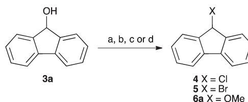
Scheme 1 Some example substitution reactions of fluorenyl 3a . (a) PBr 3 ; 14 (b) POCl 3 ; 15 (c) HCl, Δ; 16 (d) MeOH, H + , Δ. 17,18
