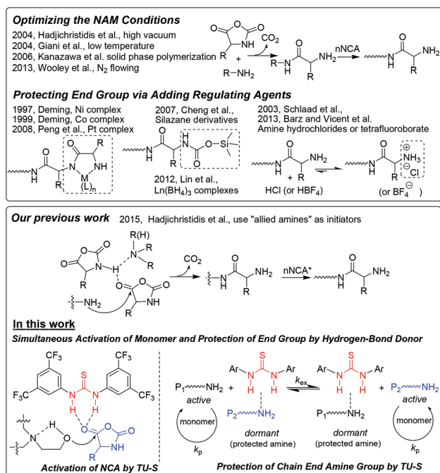
Scheme 1 Reported strategies for the living polymerization of \alpha -amino acid NCAs and the new approach proposed in this work.
