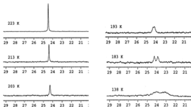
Fig. 14 VT-NMR of 3 in dichloroethane- d_2 (138–223 K).
