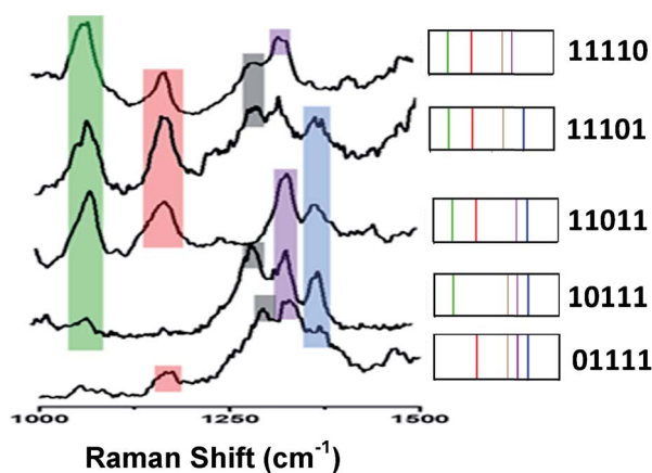
Fig. 6 Typical SERS spectra and barcode representation pictures of four type SERS labels on PS bead.
