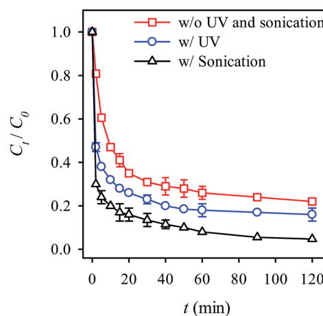
Fig. 11 Effects of UV and ultrasonication on the RB decolorization using persulfate activated by MIL-88A (persulfate = 200 \text{ mg L}^{-1} , MIL-88A = 500 \text{ mg L}^{-1} , 40 \text{ }^{\circ}\text{C} ).
