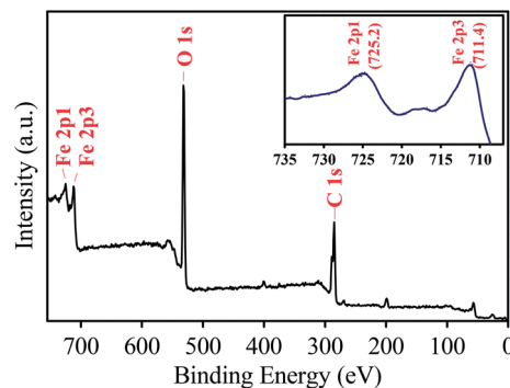
Fig. 4 XPS spectrum of full survey of the as-synthesized MIL-88A and the inset is Fe 2p core levels of MIL-88A.
