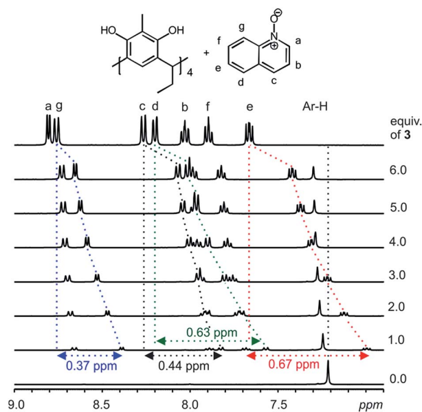
Fig. 3 ^1\text{H} NMR ( \text{CD}_3\text{OD} , 298 K) spectral changes observed from a mixture of \text{C}_2 -2-methylresorcinarene host 1 and several equivalents of quinoline N -oxide 3 . The shift changes of selected guest signals in ppm from a 1 : 1 host-guest mixture are highlighted. Vertical dotted lines gives an indication of the complexation induced shift changes.
