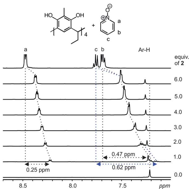
Fig. 2 ^1\text{H} NMR ( \text{CD}_3\text{OD} , 298 K) spectral changes observed from a mixture of \text{C}_2 -2-methylresorcinarene host 1 and several equivalents of pyridine N -oxide 2 . The shift changes of the guest signals in ppm from a 1 : 1 host-guest mixture are highlighted. Vertical dotted lines gives an indication of the complexation induced shift changes.
