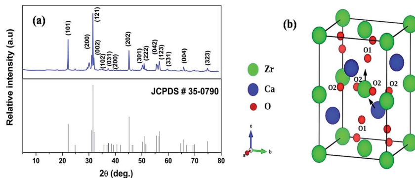
Fig. 1 (a) XRD Pattern of CaZrO 3 powder annealed at 600 °C (b) Schematic of CaZrO 3 unitcell. Arrows indicate direction of atomic displacement for the Zr and Ca network. O 1 and O 2 are the axial and planar oxygen atoms, respectively.
