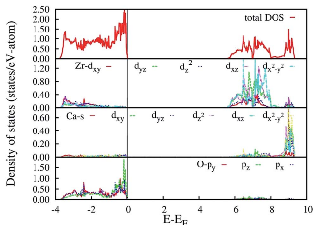
Fig. 7 HSE06 calculated total and angular momentum decomposed electronic density of states of ideal CZO (o-CZO). The vertical lines represent Fermi level.
