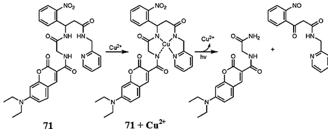
Fig. 62 Chemical structure of coucage 71, proposed copper complexation mechanism and photolysis.
