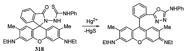
Fig. 280 Chemical structure of probe 318 and the Hg 2+ -triggered ring-opening mechanism.
