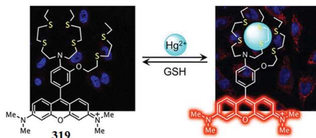
Fig. 281 Chemical structure of RosHg-based fluorescent sensor 319, its proposed binding mode with that of Hg 2+ , and reversibility in the presence of glutathione (GSH).
