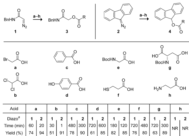
Scheme 1 Chemoselective esterification in acetonitrile.
