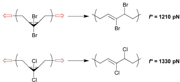
Fig. 4 g DBC and g DCC mechanophores embedded along a poly-(butadiene) backbone are activated at forces of 1210 pN and 1330 pN respectively under single molecule force spectroscopy on the time scale of \sim 0.1 s. 30 The lower force required for g DBC relative to g DCC mirrors the force-free activity.
