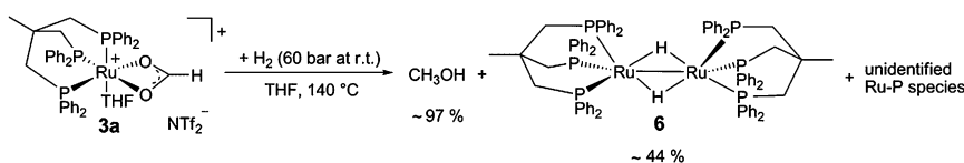
Scheme 5 Methanol is formed with high yield by hydrogenation of complex 3a .
