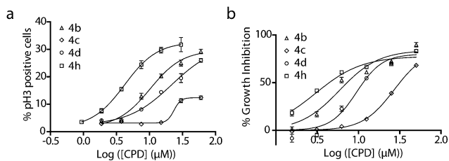
Fig. 1 Antimitotic and growth inhibitory effects of fused ring analogues 4 : (a) mitotic arrest induced by 4b–d , and 4h ; U2OS cells were incubated with compounds for 20 h before being fixed and stained with Hoechst (a DNA dye) and a pH3 specific antibody. Cells were imaged and analysed on a Cellomics Arrayscan. Data shown as the mean \pm sem for an experiment conducted in triplicate. CPD = compound; (b) Growth inhibition of U2OS cells by 4b–d , and 4h . U2OS cells were incubated with compounds for 72 h before fixing and staining with sulforhodamine B. Absorbance was then measured at 510 nm. Data is shown as the mean \pm sem for an experiment conducted in triplicate.
