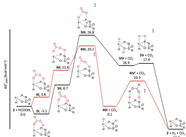
Fig. 8 Potential energy diagram (DFT, BP86, def2-TZVP) for dehydrogenation of formic acid by 5I (black profile) and 6I (red profile); \Delta G_{298K}^\ddagger is in kcal mol -1 .
