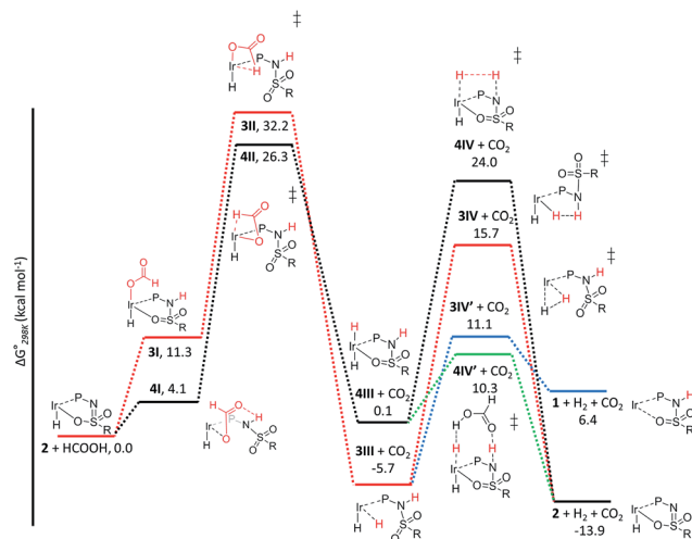
Fig. 6 Potential energy diagram (DFT, BP86, def2-TZVP) for the dehydrogenation of formic acid via \beta -hydride elimination at the equatorial (red) and axial (black) positions; \Delta G_{298K}^\ddagger is in kcal mol -1 .
