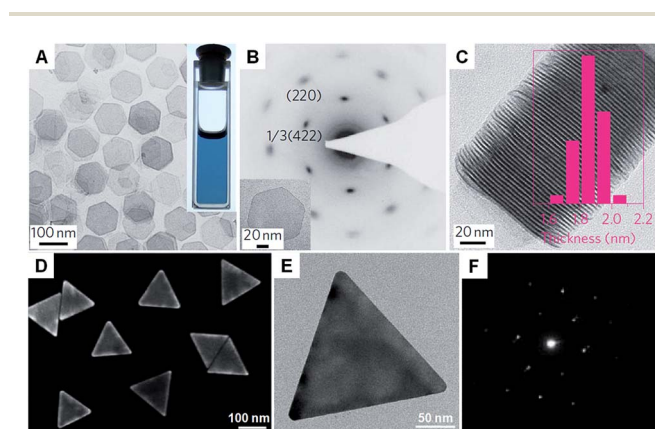
Fig. 4 (A) Bright-field TEM image of free-standing Pd nanosheets. Inset: a photograph of the Pd nanosheet solution. 29 (B) SAED pattern of a Pd nanosheet (inset) taken along the [111] zone axis. 29 (C) TEM image and the corresponding thickness analysis (inset) of the assembly of Pd nanosheets. 29 Copyright 2011, Nature Publishing Group. (D) SEM image of Au nanoprisms. 62 (E) Bright-field TEM image and (F) the corresponding SAED pattern of a typical Au nanoprism. 62 Copyright 2013, American Chemical Society.
