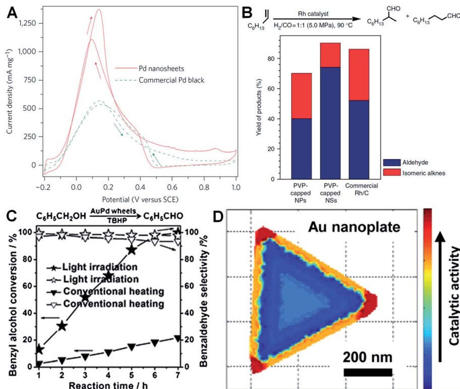
Fig. 7 (A) Cyclic voltammety (CV) curves of Pd nanosheets (edge length: 41 nm) and Pd black (Aldrich, 47 m 2 g -1 ) collected in an aqueous solution containing H 2 SO 4 (0.5 M) and HCOOH (0.25 M) at a scan rate of 50 mV s -1 . 29 Copyright 2011, Nature Publishing Group. (B) The catalytic ability comparison of PVP-capped Rh nanoparticles (NPs), PVP-capped Rh nanosheets (NSs) and commercial Rh/C in hydroformylation of 1-octene. 27 Copyright 2014, Nature Publishing Group. (C) The comparison of light irradiation (power density: 0.37 W cm -2 ) and conventional heating (temperature: 50 °C) in the selective oxidation of benzyl alcohol with Au–Pd nanowheels as the catalyst. 52 Copyright 2013, John Wiley & Sons, Inc. (D) Catalytic activity mapping of an Au nanoplate in the reductive N-deoxygenation of resazurin to resorufin by NH 2 OH, identified by the combination of single-molecule super-resolution fluorescence microscopy and electron microscopy. 163 Copyright 2013, American Chemical Society.
