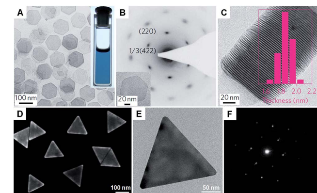
Fig. 4 (A) Bright-field TEM image of free-standing Pd nanosheets. Inset: a photograph of the Pd nanosheet solution. 29 (B) SAED pattern of a Pd nanosheet (inset) taken along the [111] zone axis. 29 (C) TEM image and the corresponding thickness analysis (inset) of the assembly of Pd nanosheets. 29 Copyright 2011, Nature Publishing Group. (D) SEM image of Au nanoprisms. 62 (E) Bright-field TEM image and (F) the corresponding SAED pattern of a typical Au nanoprism. 62 Copyright 2013, American Chemical Society.
