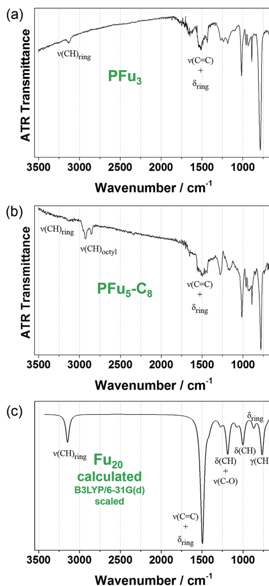
Fig. 5 Experimental FTIR-ATR spectra: (a) of P1 and (b) of P3 films electrodeposited on platinum foil. (c) DFT B3LYP/6-31G(d) calculated IR spectrum of Fu 20 (frequencies were scaled by 0.96 (ref. 31)).
