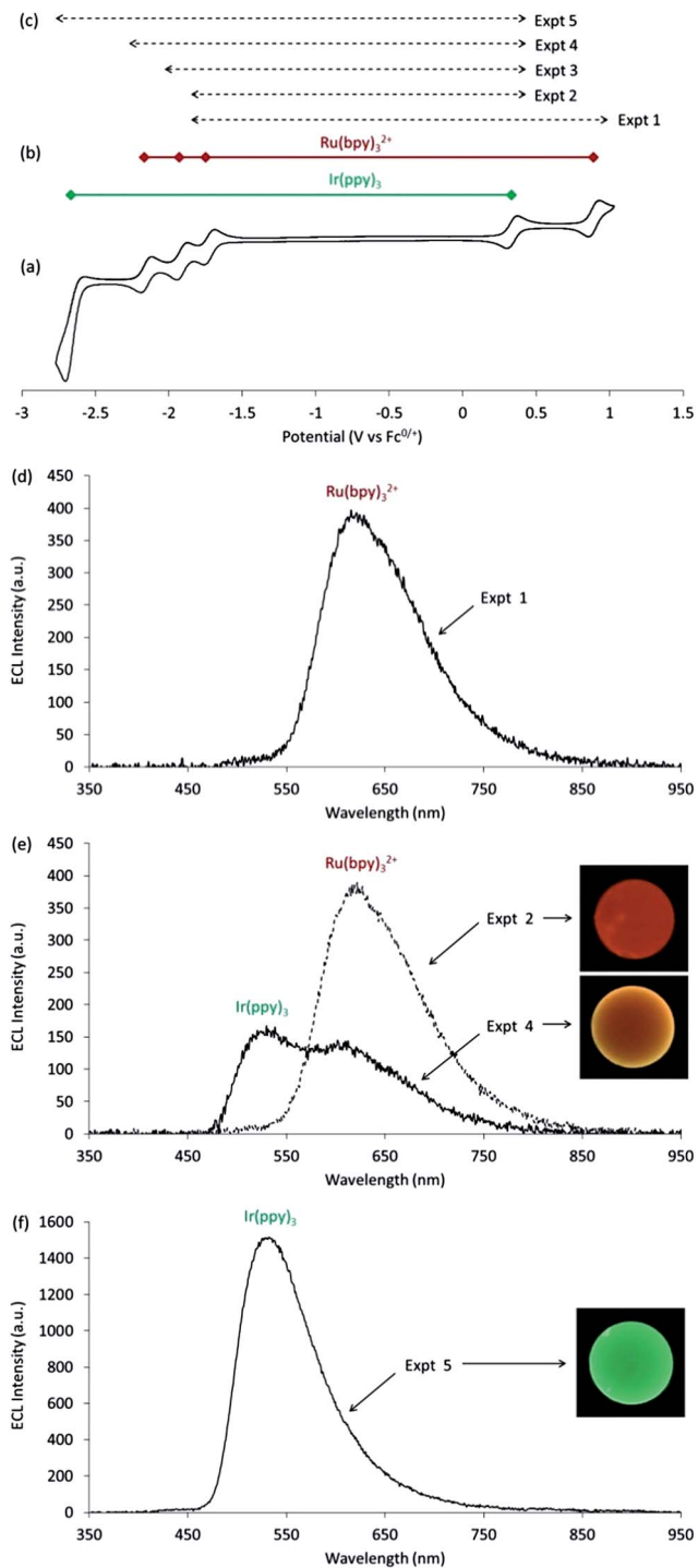
Fig. 2 (a) Cyclic voltammogram of 0.25 mM \text{Ru}(\text{bpy})_3^{2+} and 0.25 mM \text{Ir}(\text{ppy})_3 in acetonitrile containing 0.1 M TBAPF 6 . (b) Relevant reduction and oxidation potentials of the two metal chelates. (c) Illustration of potentials used in annihilation ECL experiments. (d–f) Spectra and photographs of the ECL at the working electrode of selected annihilation ECL experiments using 0.003 mM \text{Ru}(\text{bpy})_3^{2+} and 0.25 mM \text{Ir}(\text{ppy})_3 in acetonitrile containing 0.1 M TBAPF 6 .
