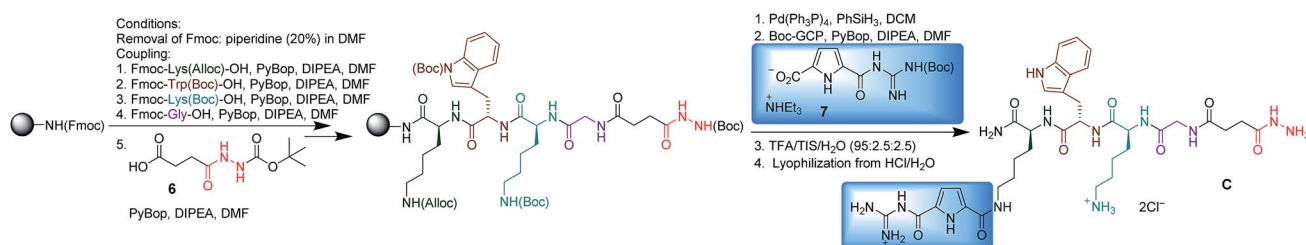
Scheme 2 Microwave assisted solid phase peptide synthesis of hydrazide C.
