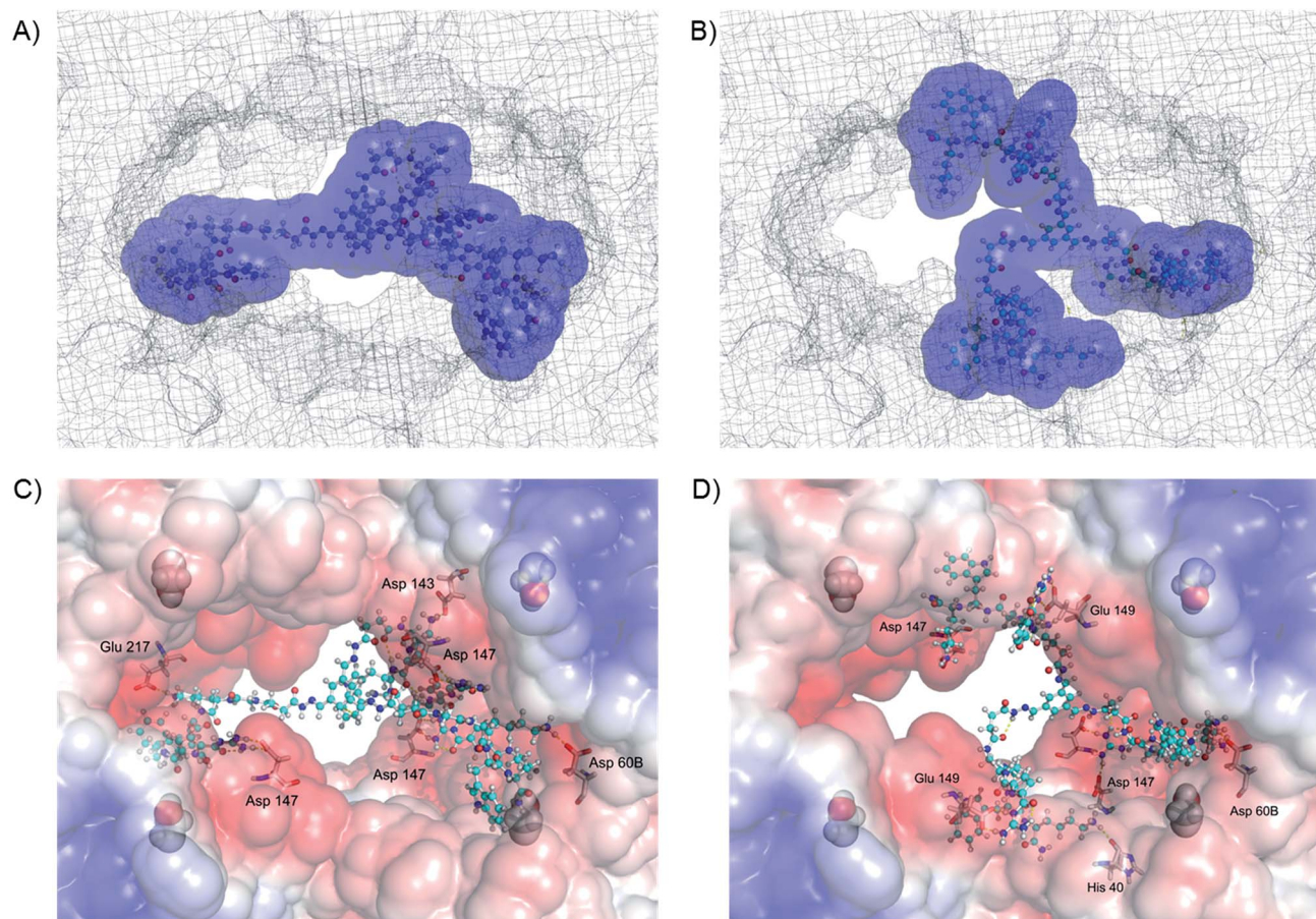
Fig. 4 Calculated binding modes of (A) inhibitor 5(\text{C})_3 (total energy of the depicted complex: -53\,717.2\text{ kJ mol}^{-1} ) and (B) inhibitor 5(\text{D})_3 (total energy of the depicted complex: -53\,683.9\text{ kJ mol}^{-1} ) to the surface (shown as mesh) of \beta -tryptase (PDB code: 1AOL). The inhibitors are shown with their accessible surface area (asa; used solvent radius 1.4\text{ \AA} for water). Close-ups of the interactions of (C) 5(\text{C})_3 (shown as balls and sticks) and (D) 5(\text{D})_3 (shown as balls and sticks) with the enzyme surface. Key protein residues (Glu, Asp and His) that interact with the inhibitors are displayed as sticks. The red, blue and grey colors on the enzyme surface indicate the negative, positive and neutral electrostatic potentials, respectively. A number of anionic residues are located around the entrance to the central pore in which the active sites are situated. Catalytic serine residues are shown using the space-filling model.
