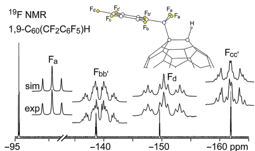
Fig. 3 Experimental and simulated 376.5 MHz 19 F NMR spectra of HPLC-purified 1,9-C 60 (CF 2 C 6 F 5 )H ( 1 ) in CDCl 3 . Chemical shifts and coupling constants are listed in Table S-2.†
