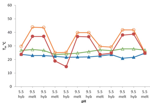
Fig. 3 Reversible assembly as a function of pH. pH variations from 5.5 to 9.5 and vice versa were achieved at 0 ^{\circ} C allowing T_m determination in hybridization (hyb)/melting (melt) cycles for T_4/B_1 (full circles), T_6/B_1 (open circles), T_4/C_1 (full triangles) and T_6/C_1 (open triangles).
