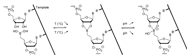
Fig. 1 DNA-templated ligation. 31
