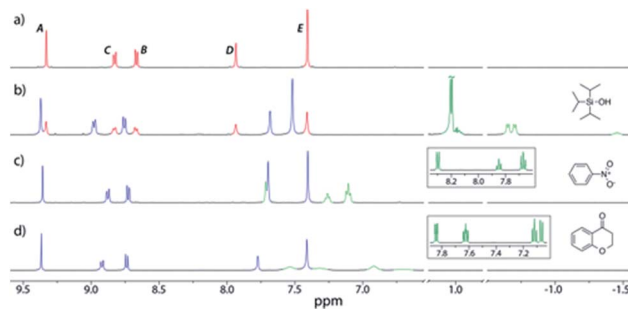
Fig. 2 Partial 1 H NMR spectra (500 MHz, D 2 O, 298 K) of (a) 2 ·12NO 3 ; (b) 2 ·12NO 3 with excess TIPSOH; (c) 2 ·12NO 3 with excess nitrobenzene; (d) 2 ·12NO 3 with excess chromanone. Color code: free capsule signals, red; bound capsule, blue; bound guest, pale green; free guest, dark green. The insets in spectra (c) and (d) show the partial 1 H NMR spectra of free guests in D 2 O. The assignments correspond to the lettering in Scheme 1.
