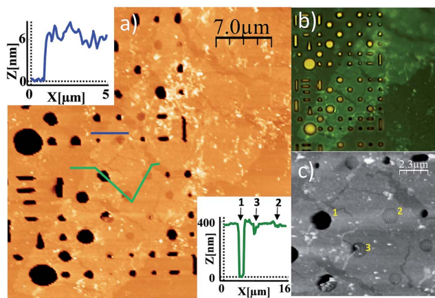
Fig. 3 Morphological characterization of the free-standing layers of [\text{Cu}(\mu\text{-pym}_2\text{S}_2)(\mu\text{-Cl})]_n \cdot n\text{MeOH} obtained on Si/SiO 2 (300 nm) substrates with wells. (a) AFM topographic image of a large suspended flake of [\text{Cu}(\mu\text{-pym}_2\text{S}_2)(\mu\text{-Cl})]_n \cdot n\text{MeOH} in an array of circular wells (400 nm depth). The topography displays the layer covering several circular wells, and the profiles taken along the flake standing on SiO 2 (blue line) and over the holes (green line), showing the areas where the sheet is suspended (2 and 3) and not suspended (1). Note how in this later case the layer completely collapses. The percentage of covered holes is about 46%. (b) Optical image of the same area than in (a). (c) Zoom area of the AFM image showing hole uncovered (1), fully covered (2) and partially covered (3) by flake of MOF [\text{Cu}(\mu\text{-pym}_2\text{S}_2)(\mu\text{-Cl})]_n \cdot n\text{MeOH} .
