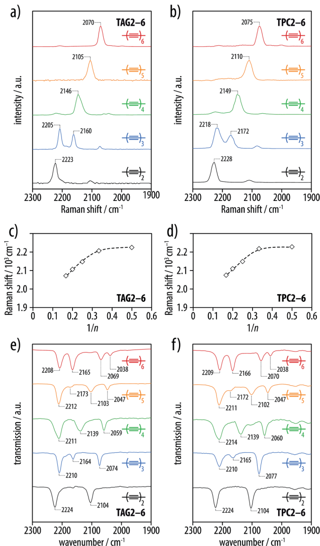
Fig. 3 IR and Raman spectra for the series of tetra- O -acetyl β-D-glucosyl oligoyne TAG2-6 and the corresponding tritylphenyl carboxylates TPC2-6. (a and b) Solid-state Raman spectra, (c and d) plots of the Raman band positions versus 1/n (the lines serve as guides to the eye), and (e and f) solid-state IR spectra of TAG2-6 and TPC2-6.
