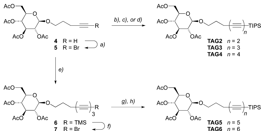
Scheme 1 Synthesis of the glycosylated oligoyne TAG2–6 up to the hexaynes. Reagents and conditions: (a) \text{AgNO}_3 , NBS, MeCN, 93%; (b) \text{TIPS-C}\equiv\text{C-ZnCl } 1 , \text{PdCl}_2(\text{dppf}) \cdot \text{DCM} , THF/toluene, 87%; (c) \text{TIPS-(C}\equiv\text{C)}_2\text{-ZnCl } 2\text{a} , \text{PdCl}_2(\text{dppf}) \cdot \text{DCM} , THF/toluene, 78%; (d) \text{TIPS-(C}\equiv\text{C)}_3\text{-ZnCl } 3 , \text{PdCl}_2(\text{dppf}) \cdot \text{DCM} , THF/toluene, 51%; (e) \text{TMS-(C}\equiv\text{C)}_2\text{-ZnCl } 2\text{b} , \text{PdCl}_2(\text{dppf}) \cdot \text{DCM} , THF/toluene, 72%; (f) \text{AgF} , NBS, MeCN, 81%; (g) \text{TIPS-(C}\equiv\text{C)}_2\text{-ZnCl } 2\text{a} , \text{PdCl}_2(\text{dppf}) \cdot \text{DCM} , THF/toluene, 42%; (h) \text{TIPS-(C}\equiv\text{C)}_3\text{-ZnCl } 3 , \text{PdCl}_2(\text{dppf}) \cdot \text{DCM} , THF/toluene, 55%.
