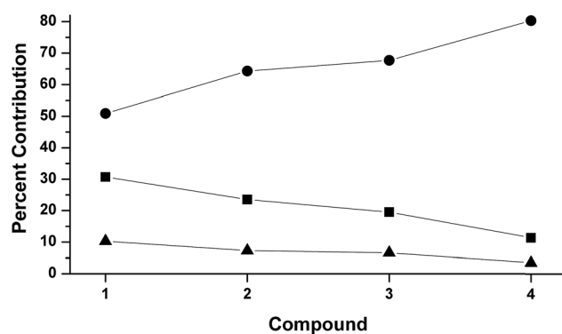
Fig. 5 DFT-derived (B3LYP, Loewdin population analysis) percent contribution to the molecular LUMOs of complexes 1–4 from L 2 ( O_2 , PhNO , ArF_2N_2 , styrene; ●), d_{xz} (■), and the two nitrogens of [R_2NN] (▲).
