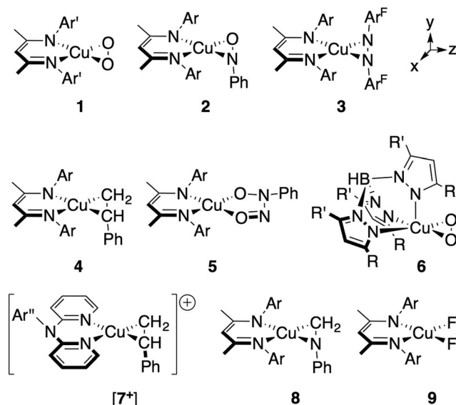
Fig. 2 Depictions of compounds 1 – 9 ; the connectivity is not intended to reflect the ground state electronic structures (see text). The following abbreviations were used: Ar = 2,6-( \text{CH}_3 ) 2 - \text{C}_6\text{H}_3 ; Ar' = 2,6-[ \text{CH}(\text{CH}_3) ] 2 - \text{C}_6\text{H}_3 ; Ar F = 3,5-( \text{CF}_3 ) 2 - \text{C}_6\text{H}_3 ; R = \text{C}(\text{CH}_3) 3 , adamantyl; R' = \text{CH}(\text{CH}_3) 2 ; Ar'' = 2-( \text{CH}(\text{CH}_3) ) 2 - \text{C}_6\text{H}_4 .
