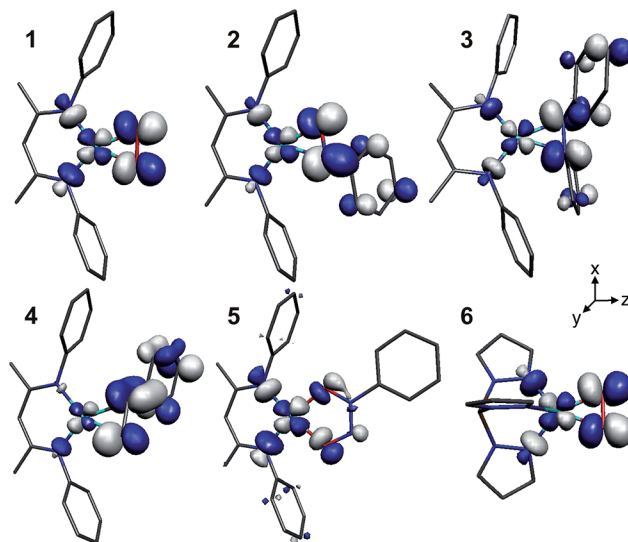
Fig. 4 Graphical representations of the DFT-derived LUMOs for complexes 1–6 . The [^iPr_2NN] ( 1 ), [Me_2NN] ( 2–5 ), and Tp' ( 6 ) ligands have been graphically truncated for clarity.
