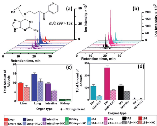
Fig. 2 Single reaction monitoring (SRM) LC-MS chromatogram for m/z transition 299–152 monitoring formation of O^6 -pyridyloxylbutyl-guanine ( 4 , Scheme 4) adducts from biocolloid reactors (enzyme color code on bottom) featuring (a) human organ microsomes, (b) cyt P450 supersomes; (c) and (d) are total DNA adducts found (pmol (\mu\text{g of protein})^{-1} (\text{mM of NNK})^{-1} ) after reactions with 150 \mu\text{M} NNK at pH = 7.4 for 18 h, (c) human organ microsomes, (d) cyt P450 supersomes.
